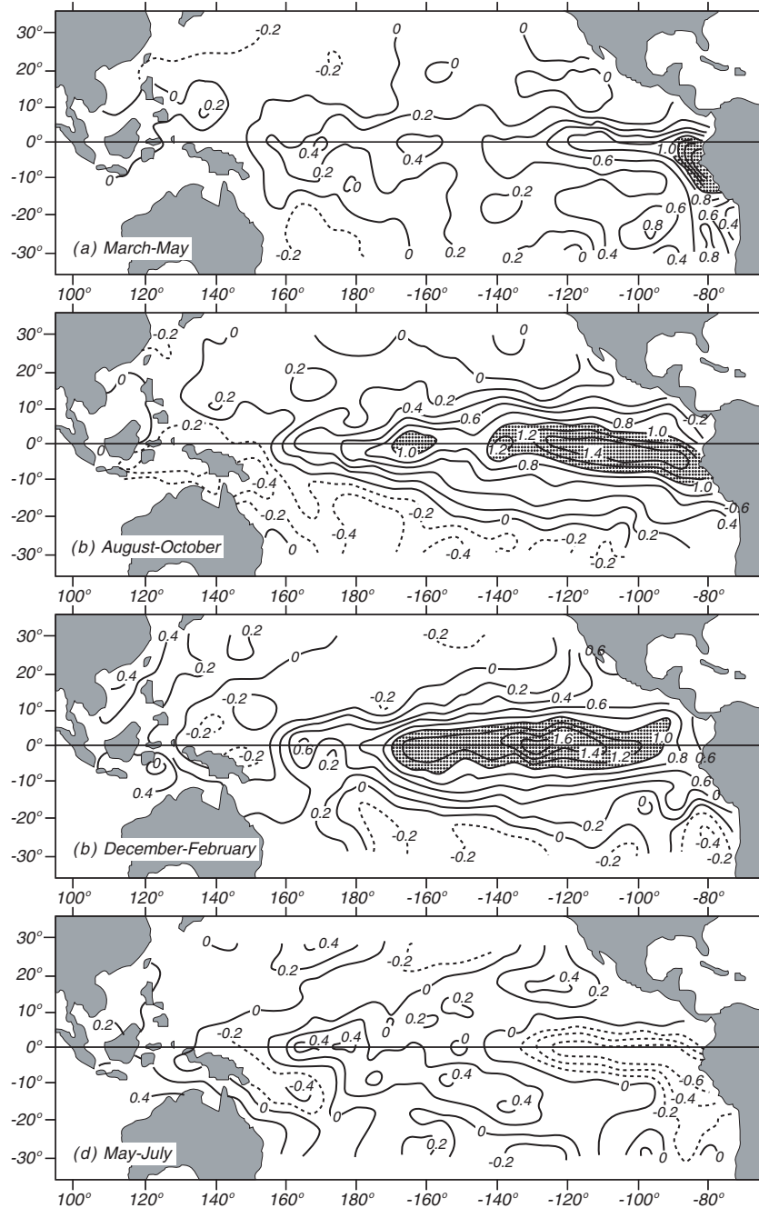
Figure 14.8 Anomalies of sea-surface temperature (in °C) during a typical El Niño obtained by averaging data from El Niños between 1950 and 1973. Months are after the onset of the event. After Rasmusson and Carpenter (1982).
