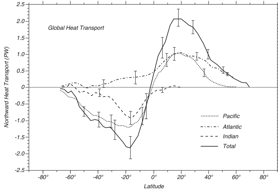
Figure 5.11 Northward heat transport for 1988 in each ocean and the total transport summed over all oceans calculated by the residual method using atmospheric heat transport from ECMWF and top of the atmosphere heat fluxes from the Earth Radiation Budget Experiment satellite. After Houghton et al. (1996: 212), which used data from Trenberth and Solomon (1994). 1 PW = 1 petawatt = 10^{15} W.
